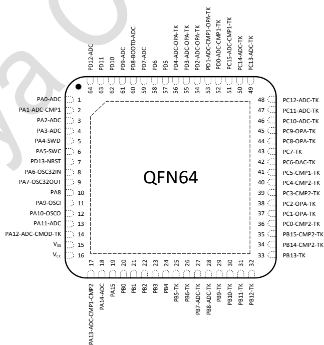
图 3-2 QFN64 PY32T090R2xU7-E Pinout2 (Top view)
